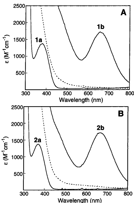
Figure 1. Electronic absorption spectra for the formation of dioxxygen adducts of diiron(II) complexes in CH 2 Cl 2 at -78 °C and their thermal decay products (---): (A) [Fe 2 (μ-O 2 CAr Tol ) 2 (O 2 CAr Tol ) 2 (C 5 H 5 N) 2 ] ( 1a ); (B) [Fe 2 (μ-O 2 CAr Tol ) 4 (4- t BuC 5 H 4 N) 2 ] ( 2a ).
